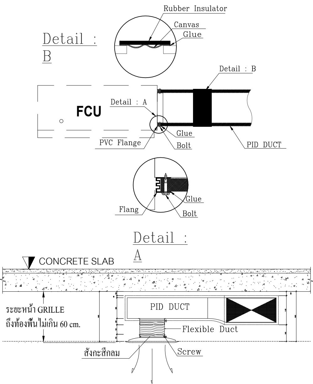
MACHINE CONNECTION
