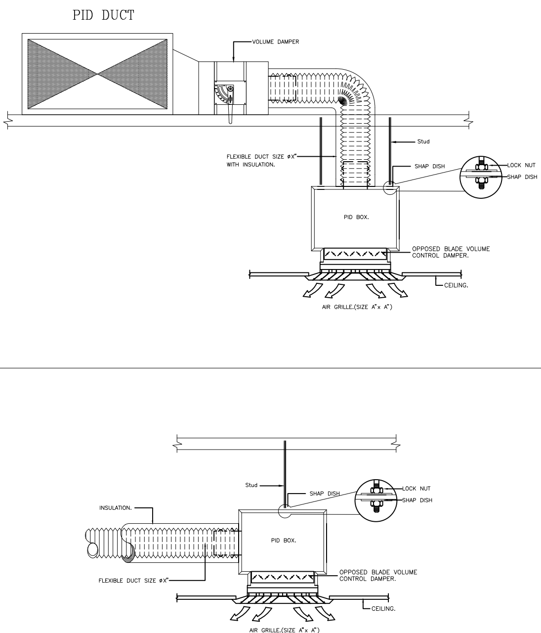
INSTALLATION DUCT
