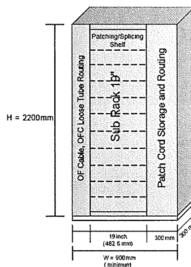
Figure 1 Dimension and allocation of FDF
